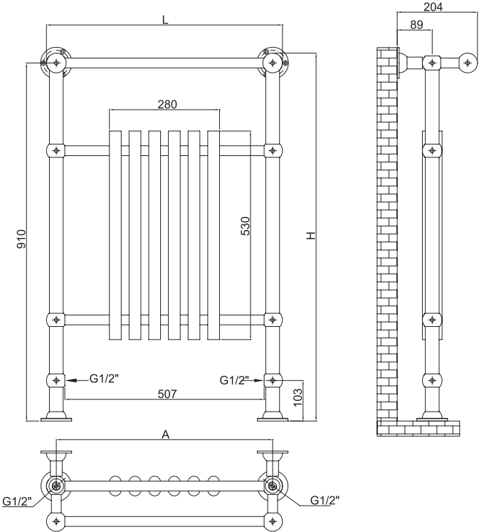
Hydraulic connections/ Conexiuni hidraulice*
